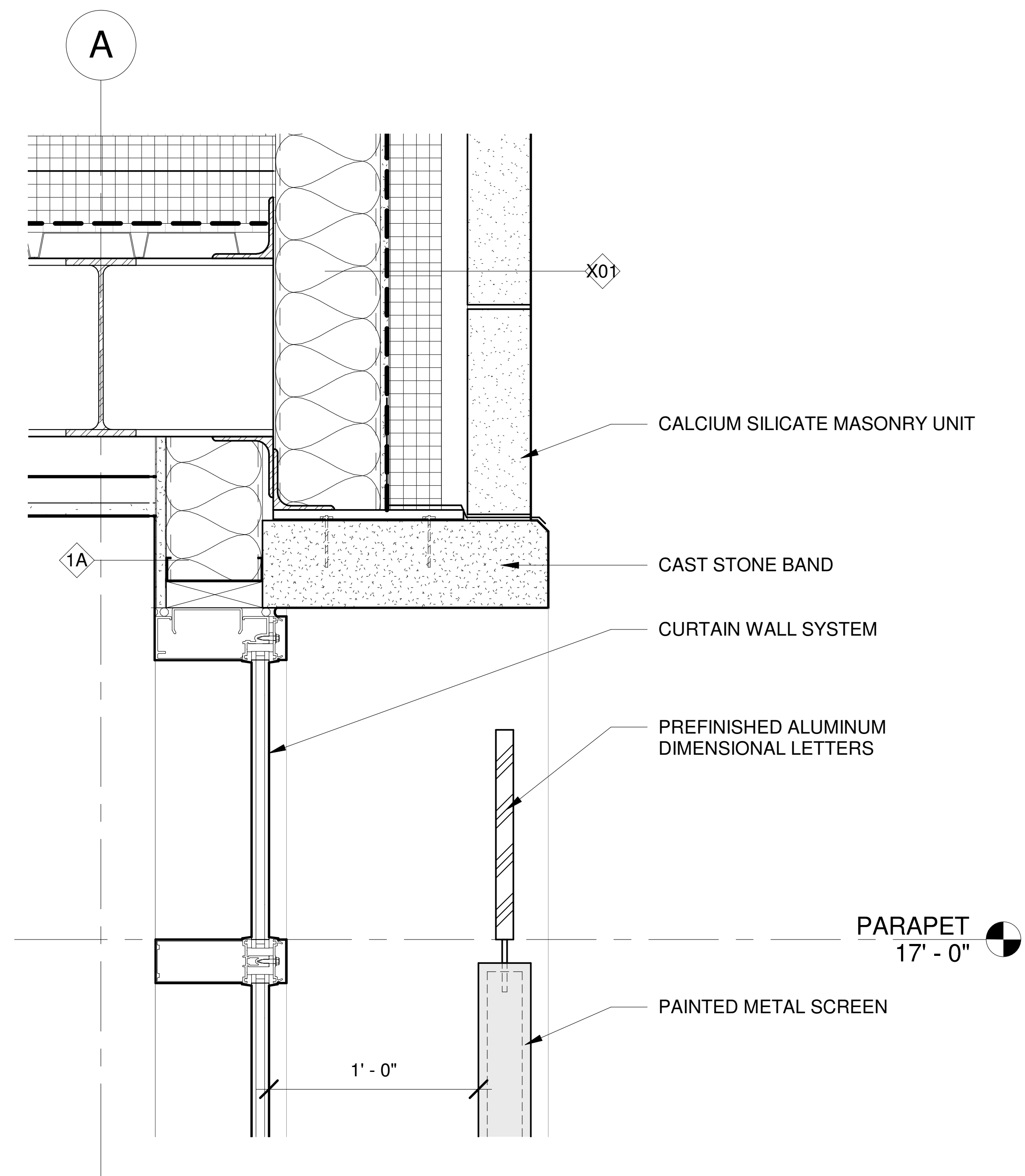
SECTION DETAIL - ADDITION ENTRY 1 1/2" = 1'-0"
